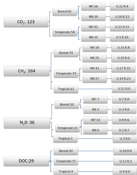
Figure 3. Number of data entries (see main text for inclusion criteria) used to derive carbon dioxide (CO 2 ), methane (CH 4 ), nitrous oxide (N 2 O) and dissolved organic carbon (DOC) emission factors. Entries are disaggregated by climate zone (boreal, temperate and tropical), nutrient status (NP = nutrient poor, NR = nutrient rich) and drainage status (U = undrained, R = rewetted).
